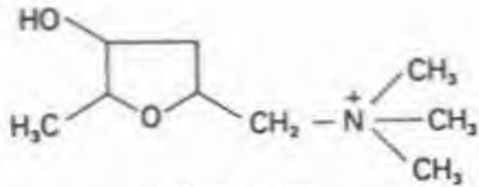
MUSCARINE
